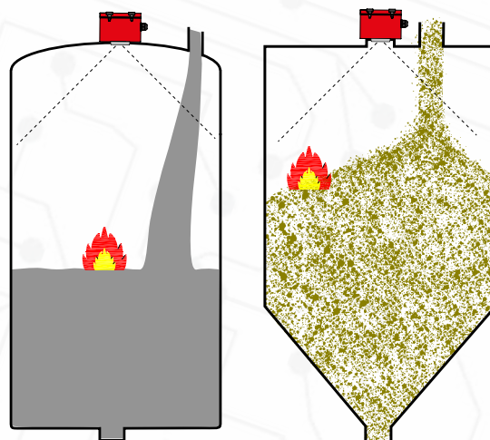
Example of installation on tanks/silos with GMSUP2-EX-TU
